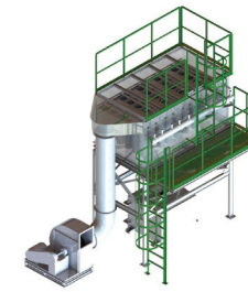
Centrifugation Type Cyclone
